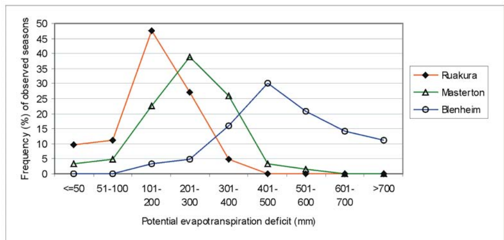
Figure 6.10.1 Frequency (%) of July to June seasons at various levels of potential evapotranspiration deficit, ranging from the wettest site at Ruakura, to progressively drier distributions at Masterton and Blenheim.
