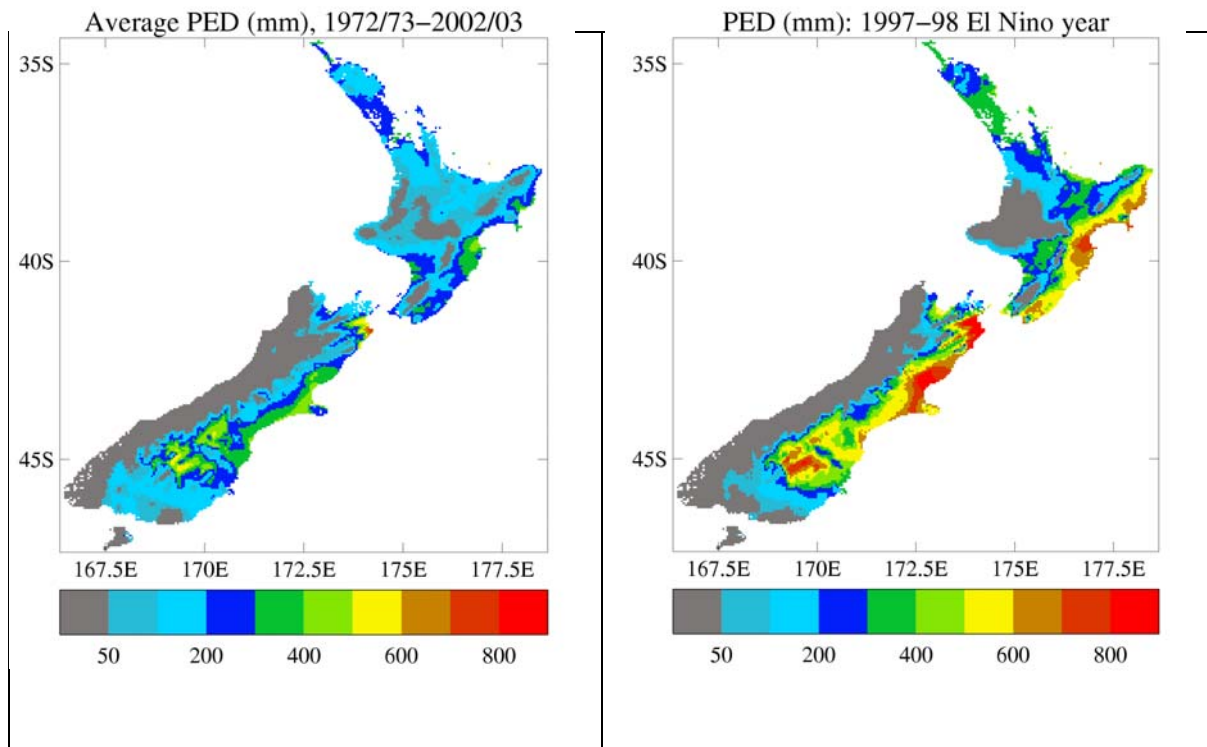
Figure 2.1 Accumulated July-June PED (mm) calculated from 0.05° gridded data set: average over 31-year period 1972/73 to 2002/03 (left), and PED levels in extreme drought year of 1997/98 El Niño (right).
