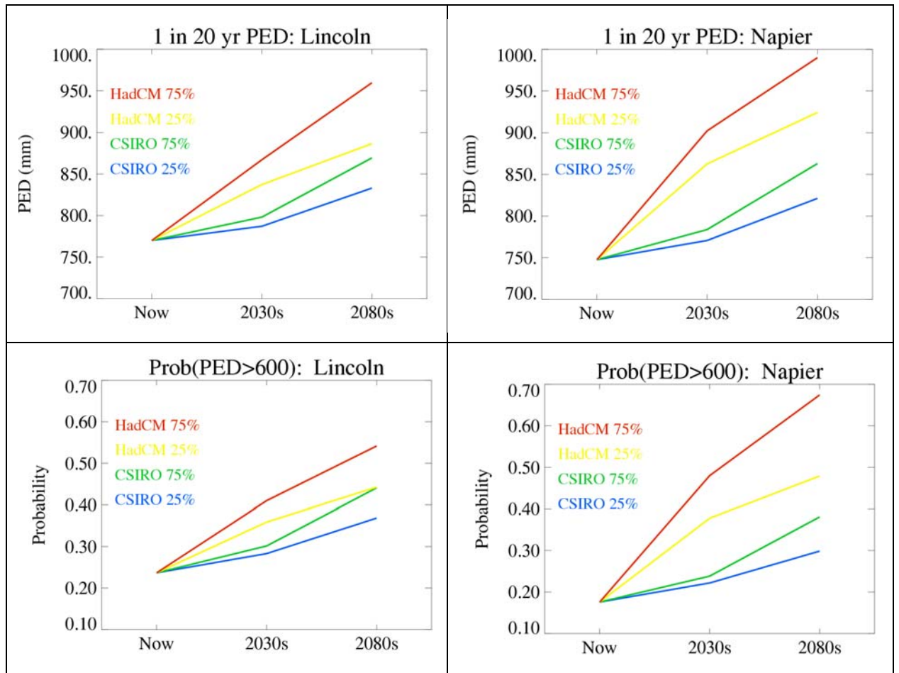
Figure 3.3 Scenario variation of annual PED at the Lincoln and Napier gridpoints. Results are shown for the current climate (“Now”), the 2030s, and the 2080s, for four scenarios. The two upper panels show PED levels with a 1-in-20 year return period (5% chance of occurrence in any one year), and the two lower panels show probabilities of annual PED exceeding 600mm. For context, the worst droughts in the recent historical record had 851mm PED at Lincoln (in 1988/89), and 799mm at Napier (1997/98).
