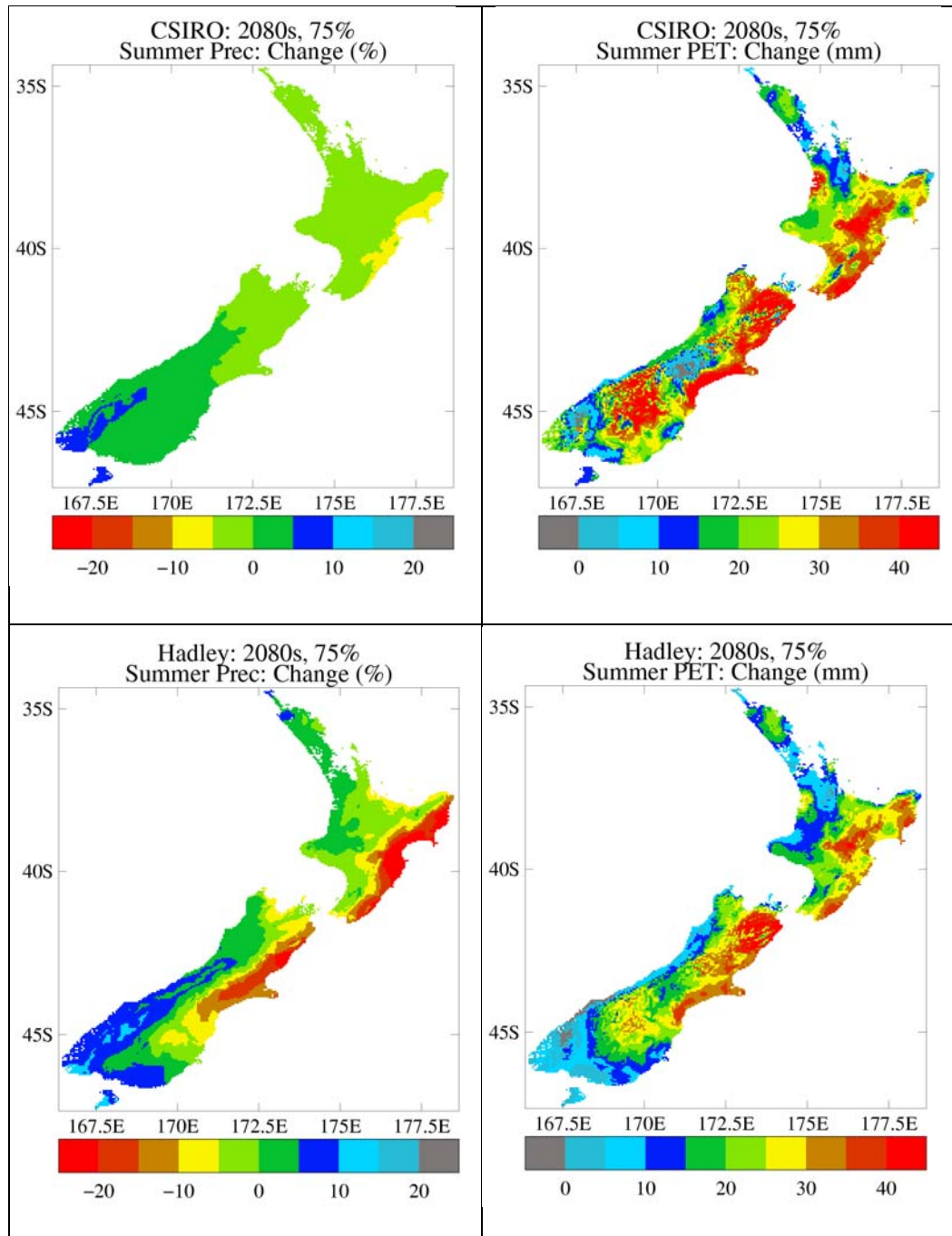
Figure 1.1 Climate change scenarios for the 2080s, with 75% IPCC scaling, for summer precipitation (%) and summer total potential evapotranspiration (mm), from downscaling the CSIRO and Hadley model output.
