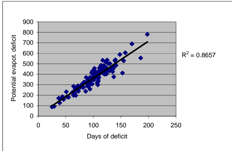
Figure 6.3.1 Relation between the potential evapotranspiration deficit (in mm) and the number of days on which an evapotranspiration deficit occurred, calculated with the method shown in Appendix (section 6.3), for Lincoln, July to June seasons from 1881/82 to 2003/04.
