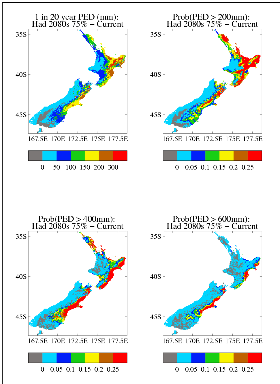
Figure 6.9.4 As Figure 6.9.3, but for the Hadley 2080s 75% scenario.
