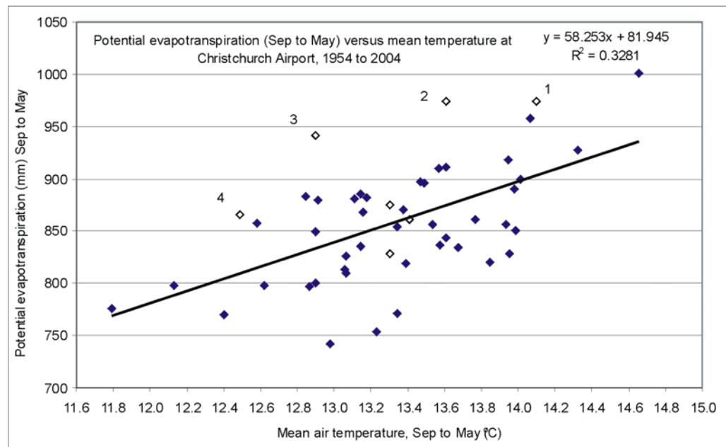
Figure 6.5.1 Apparent relationship between seasonal (September to May) mean air temperature and calculated potential evapotranspiration ( PET ) at Christchurch Airport, 1954-55 to 2003-04. The highest PET (1001 mm) occurred in warmest year, the La Niña season of 1988-89. Open points are El Niño years; enumerated points are referred to in the text. The trendline is indicative only.
