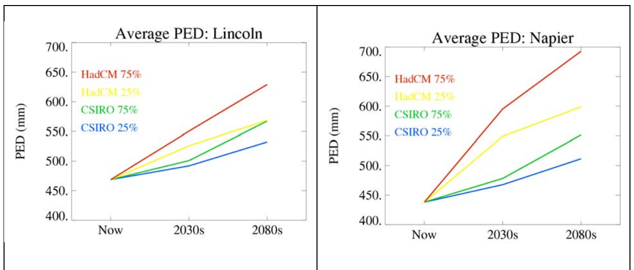
Figure 3.2 Average annual accumulated PED (in mm) at two gridpoints corresponding to Lincoln and Napier. Results are shown for the current climate (“Now”), the 2030s, and the 2080s, for four climate change scenarios.
