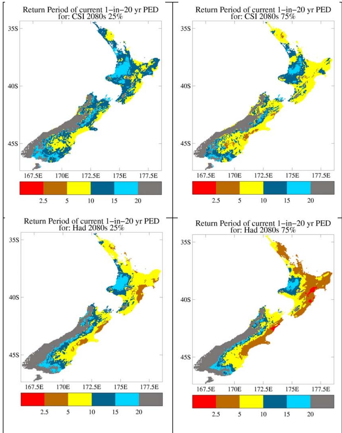
Figure 3.4: Future return periods (years) of current climate 1-in-20 year PED events, for four scenarios: CSIRO 2080s 25% and 75% scaling (upper panels) and Hadley 2080s 25% and 75% scaling (lower panels). Grey areas indicate regions of very low drought risk (where return period can't be estimated) and/or regions where drought risk decreases.
