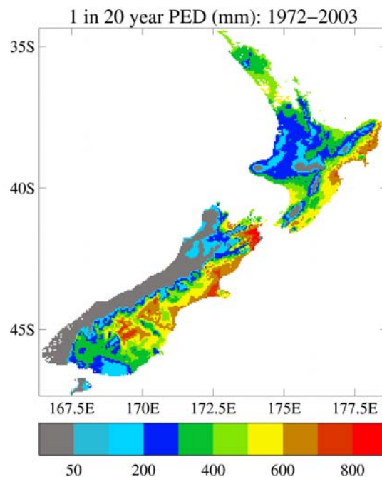
Figure 2.4 PED (mm) with a 1 in 20 year return period, equivalent to a 5% chance (or probability of 0.05) of occurrence in any one year.
