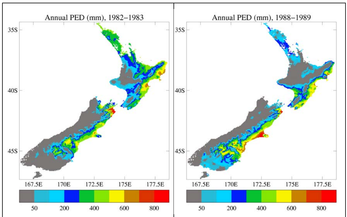
Figure 6.8.3 Annual PED accumulation (mm) for two severe drought years: 1982/83, a strong El Niño; and 1988/89, the worst drought on record at Lincoln.
