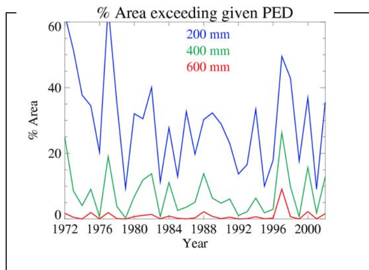
Figure 2.2 Fraction of gridpoints (on 0.05° grid) with July-June PED accumulation exceeding specified threshold. The time series highlights the severe droughts.
