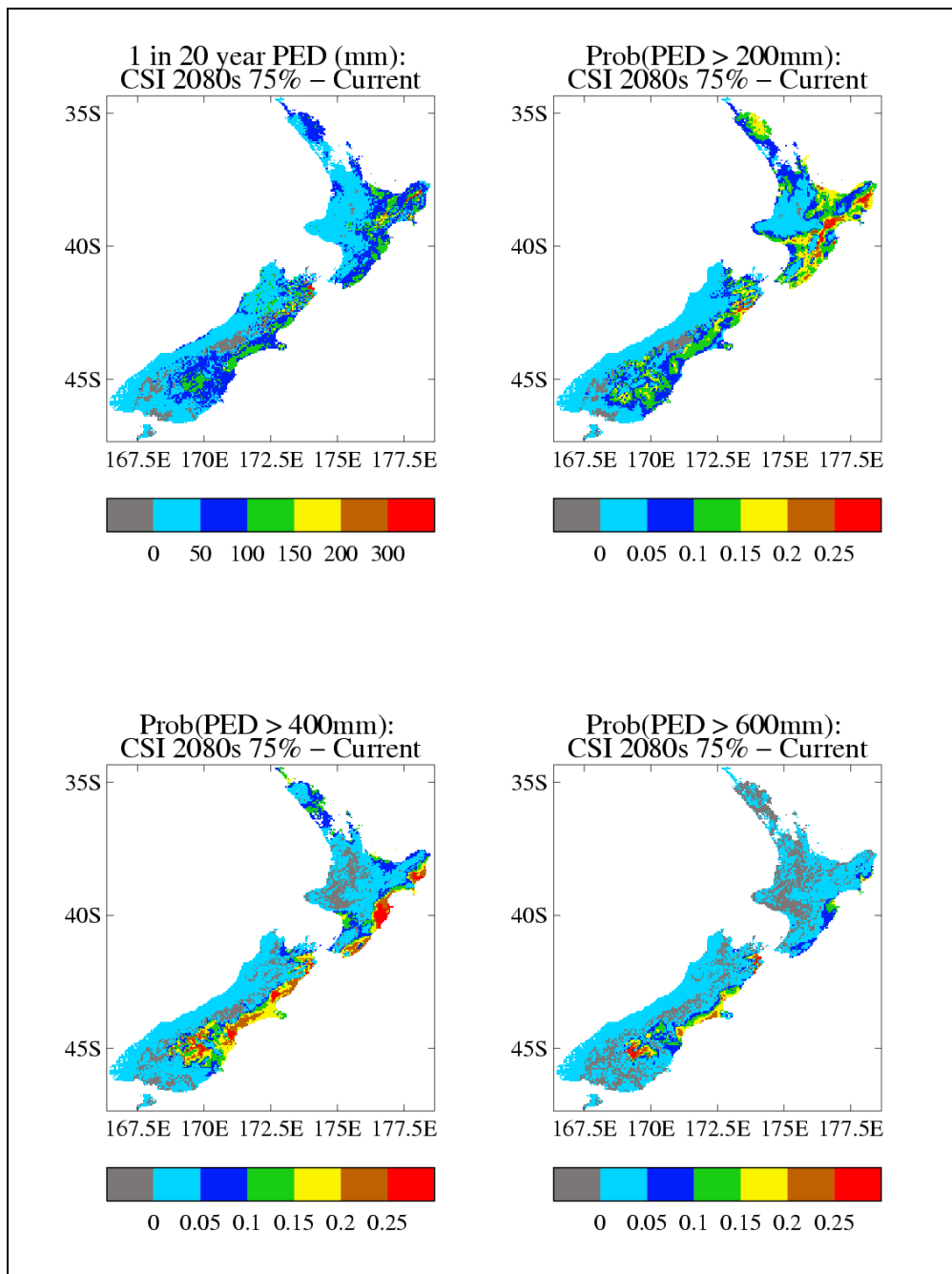
Figure 6.9.3 Change in drought statistics from the present for the CSI 2080s 75% scenario.
