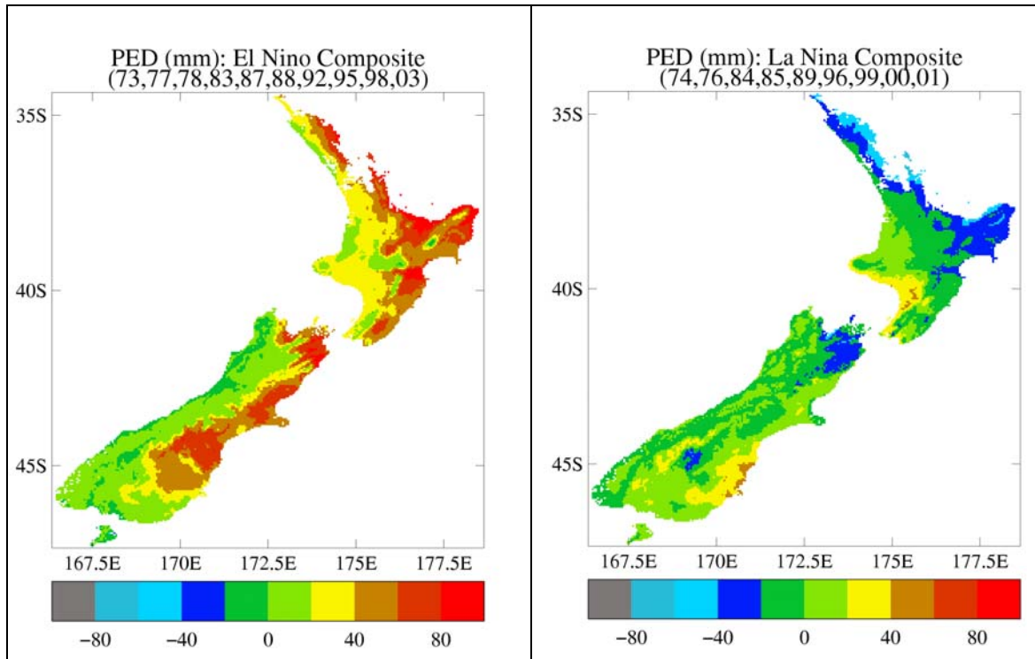
Figure 6.7.1 Average July-June PED (mm) composited over El Niño and La Niña periods. The years used in the composite (eg, 1972/73 is first El Niño year) are chosen according to the state of the El Niño-Southern Oscillation over Dec-Feb season.
