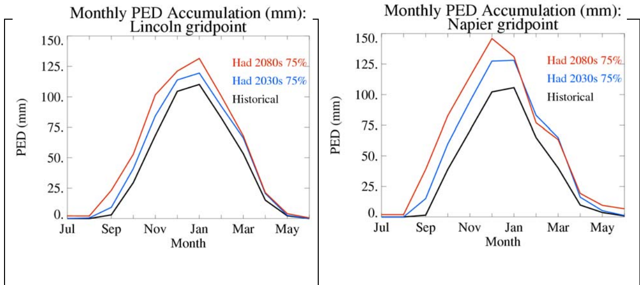
Figure 3.5 Monthly accumulation of PED (in mm) at the Lincoln (left) and Napier (right) gridpoints, comparing historical distributions with those projected by Hadley model with IPCC 75% scaling.
