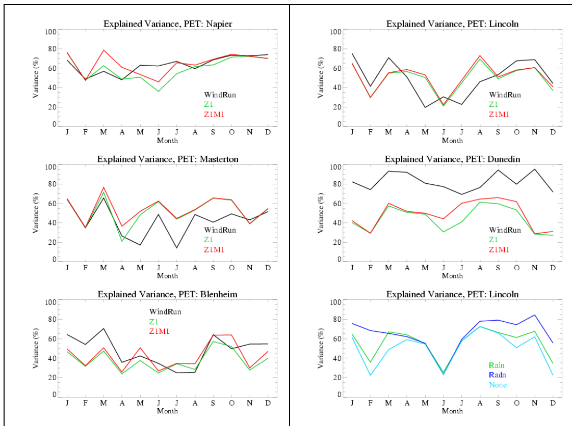
Figure 6.5.2 Explained variance (%) of monthly PET from multiple linear regression estimates. First five panels show effect of replacing station windrun with a pressure index. Last panel (lower right) shows effect of using rainfall as proxy for solar radiation at Lincoln.
