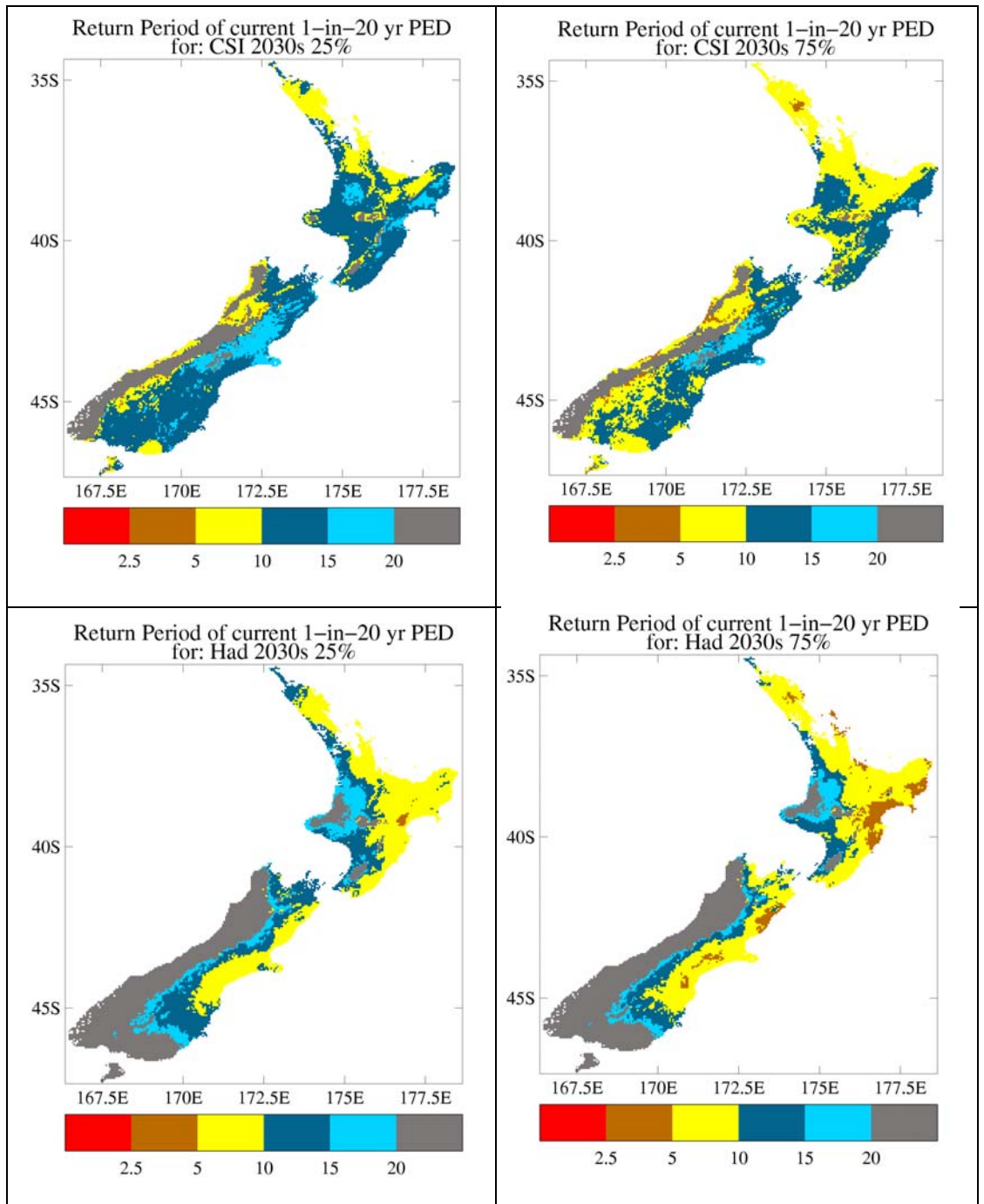
Figure 6.9.5 Future return periods (years) of current climate 1-in-20 year PED events, for four scenarios: CSIRO 2030s 25% and 75% scaling (upper panels) and Hadley 2030s 25% and 75% scaling (lower panels). This is the equivalent of Figure 3.4, but for the 2030s instead of the 2080s.
