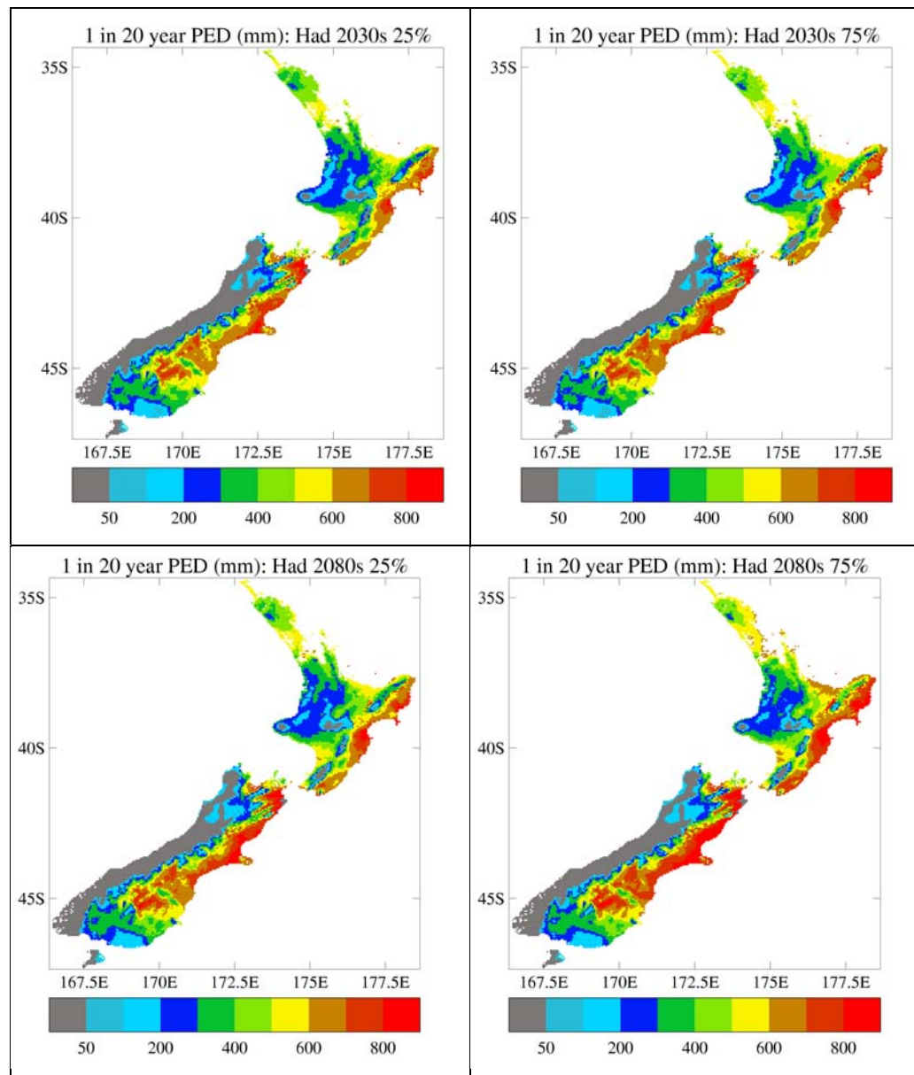
Figure 6.9.2 As Figure 6.9.1, but for the Hadley model.
