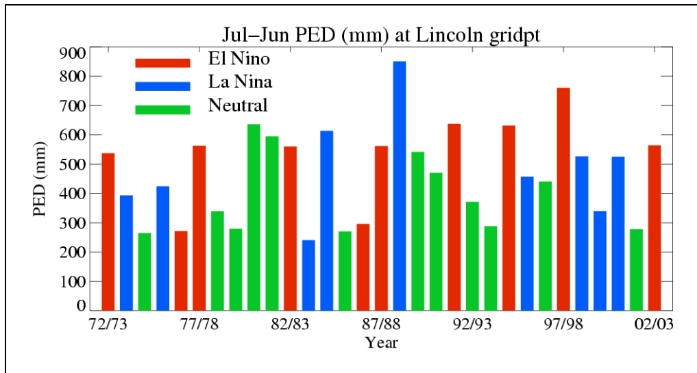
Figure 6.8.2 Accumulated July-June PED (mm) at the gridpoint closest to Lincoln, 1972/73 to 2002/03, extracted from the 0.05° gridded data set. Bars are coloured according to El Niño/La Niña status over the summer season.
