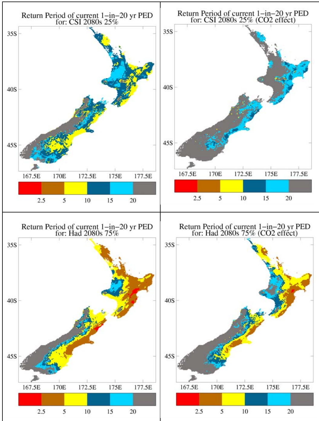
Figure 6.11.1 Future return periods (years) of current climate 1-in-20 year PED events, for four scenarios: CSIRO 2080s 25% scaling (top) and Hadley 2080s 75% scaling (bottom), and for standard scenario (left) and with ad hoc 5% PET reduction to represent increased stomatal resistance under CO 2 enrichment (right).
