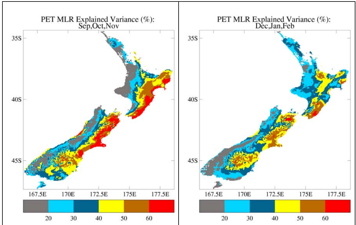
Figure 6.5.3 Percentage of variance explained by the PET multiple linear regression for: the three spring months (left panel) and three summer months (right panel) combined.
