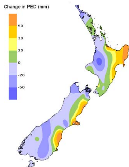
Figure 6.7.2 Mean change in July-June PED (in mm) after the 1977/78 season, compared to previous seasons from 1950/51.
