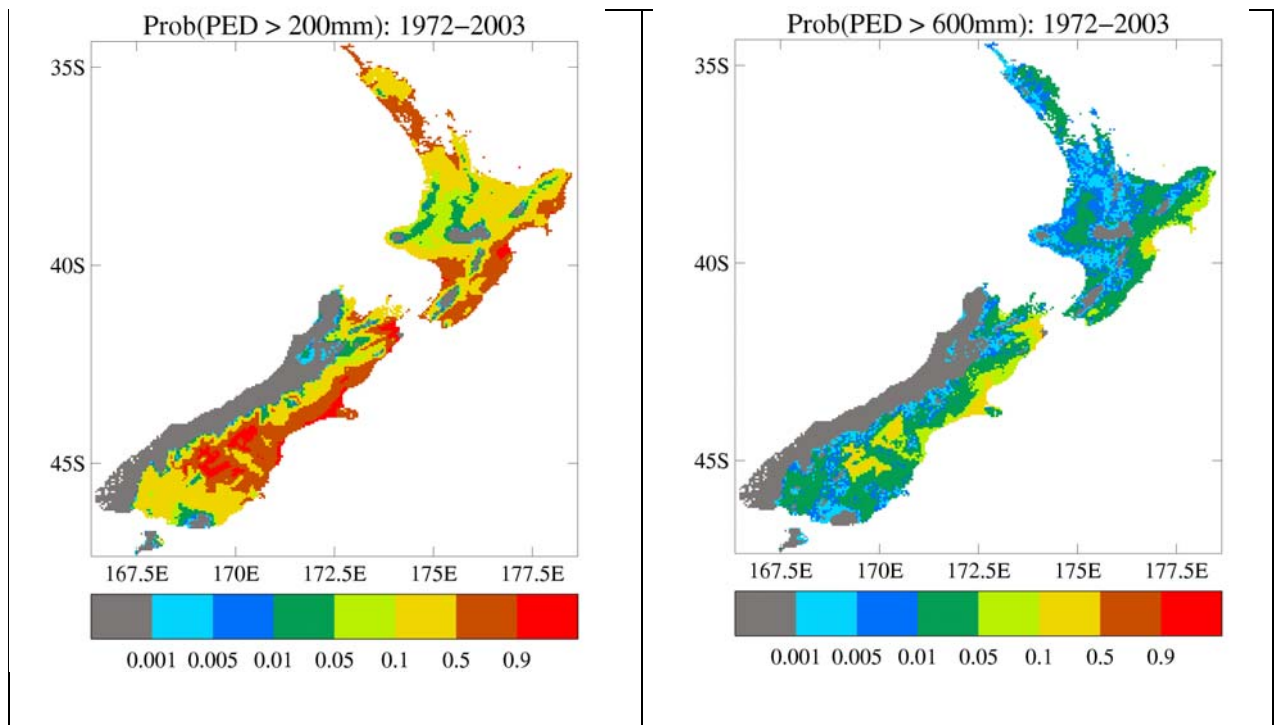
Figure 2.3 Probability that in any one year the annual accumulated PED will exceed 200 mm (left) and 600 mm (right). The inverse of the probability gives the return period of the specified deficit. For example, a probability of 0.05 corresponds to a return period of 20 years.
