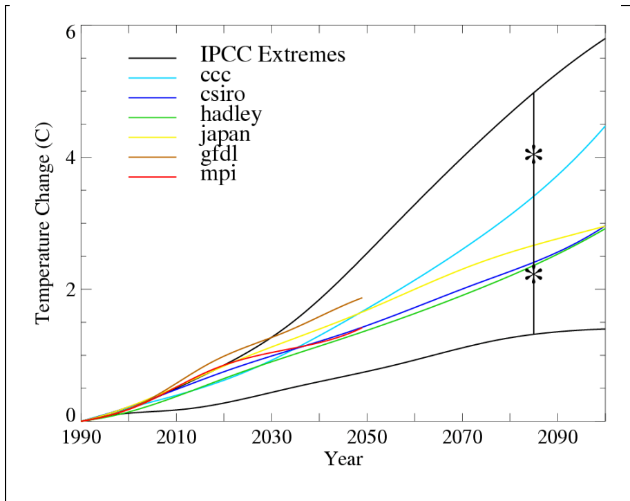
Figure 6.6.1 Global-mean surface temperature changes from a range of models (coloured lines), and the IPCC extreme range (black lines). Stars on the vertical bar at 2085 indicate schematically the IPCC 25 percentile and 75 percentile for the 2080s. Note that in practice (see text) we use a 30-year period, not a single year, and calculate the quartiles of the extreme low to high scaling factor range, not quartiles of the temperature change.
