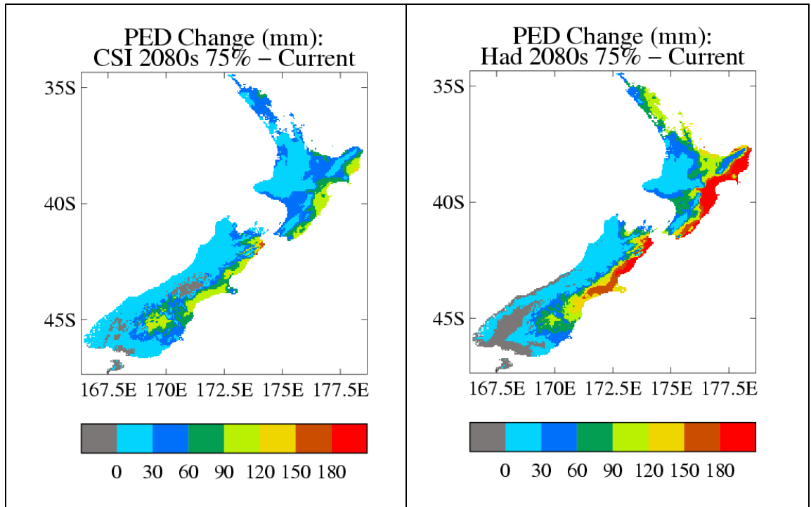
Figure 3.1 Average change in annual accumulated PED (in mm) between the current climatology and projected climatology for the 2080s according to the CSIRO (left) and Hadley (right) models, scaled to the IPCC 75% global warming. The contour intervals, every 30mm, correspond approximately to one week of pasture evapotranspiration deficit in summer.
