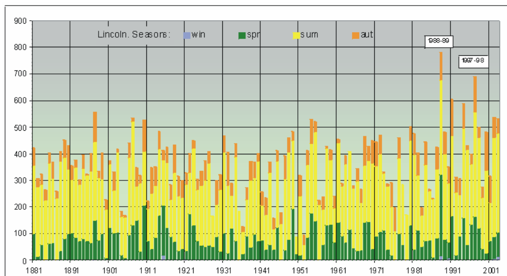
Figure 6.8.1 Accumulated June-May PED (mm) at Lincoln, 1881/82 to 2003/04, using data obtained from the NIWA Climate Database. Three-month seasonal accumulations are separated according to colour on each bar. The series highlights 1988/89 and 1997/98 as the most severe droughts in the past 122 years. These two seasons were associated with a strong La Niña and El Niño event respectively. (Figure 1 in Phase 1 report, Porteous, 2004).
