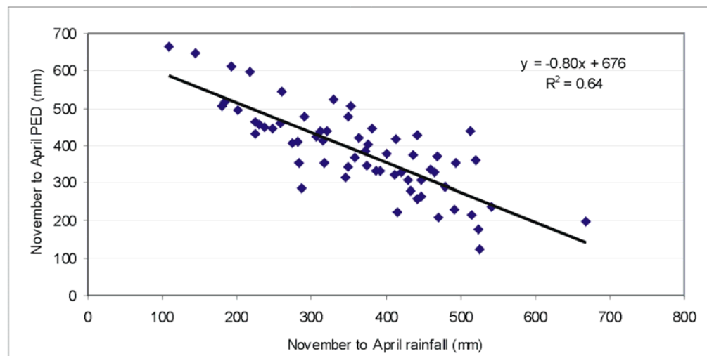
Figure 6.4.1 Dependence of November to April PED on rainfall for the same period, at Napier (Nelson Park site).
