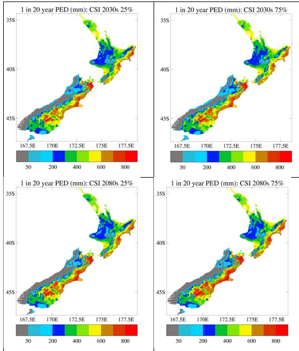
Figure 6.9.1 PED (mm) with a 1 in 20 year return period (5% chance of occurrence in any one year) for the four future scenarios based on the CSIRO model.
